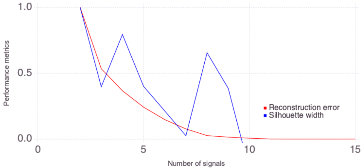
Figure 2: Estimated reconstruction error O(k) and silhouette width S(k) for different numbers of signals k .
